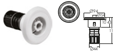
Dz Grnml (Standart) Jet Smooth Face (Swirl Jet)
