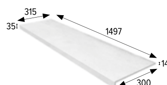
Straight stair-tread 180
